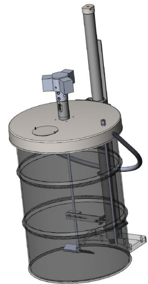
3099-5520-000 - 55 Gallon Direct Drive Agitator with Elevator and Drum Lid
