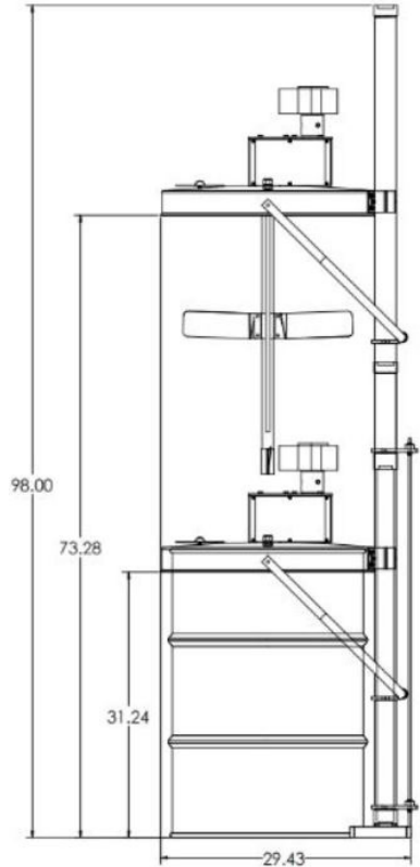
Width of unit approximately 27.5
