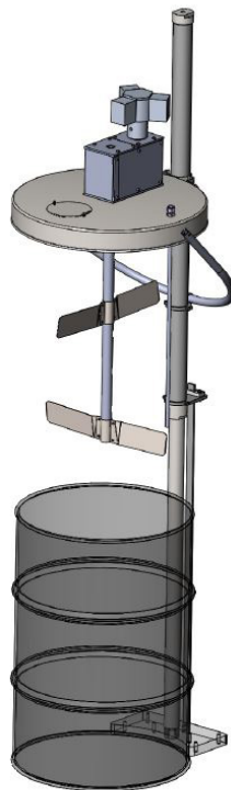
3092-BG55-000 - 55 Gallon Back Geared Agitator with Elevator and Drum Lid
