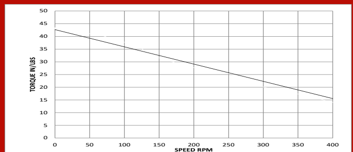
@ 50 psi size 3 motor
