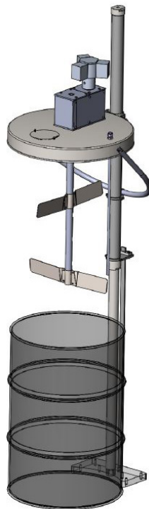
3092-BG55-100 - 55 Gallon Back Geared Agitator with Elevator and Drum Lid
