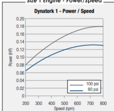
Size 1 Engine - Power/Speed
