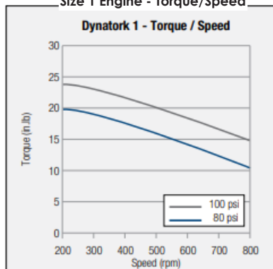
Size 1 Engine - Torque/Speed
