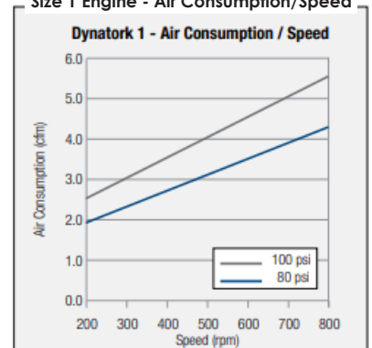
Size 1 Engine - Air Consumption/Speed
