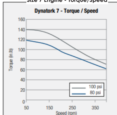
Size 7 Engine - Torque/Speed
