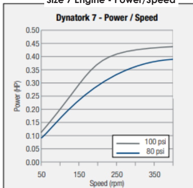
Size 7 Engine - Power/Speed
