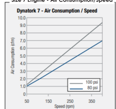
Size 7 Engine - Air Consumption/Speed
